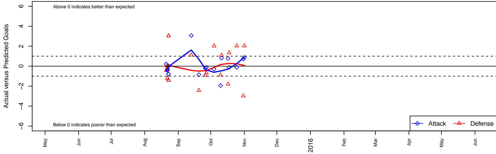
LCYSA Osprey B01 Dots are actual minus expected GF (blue circles) and GA (red triangles). Blue line is smoothed change in attack strength. Red is smoothed change in defense strength.
